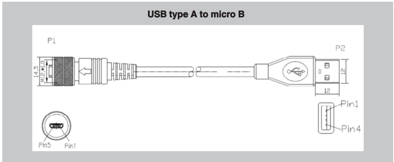
Figure 5.6.2B USB type A to micro B cable
