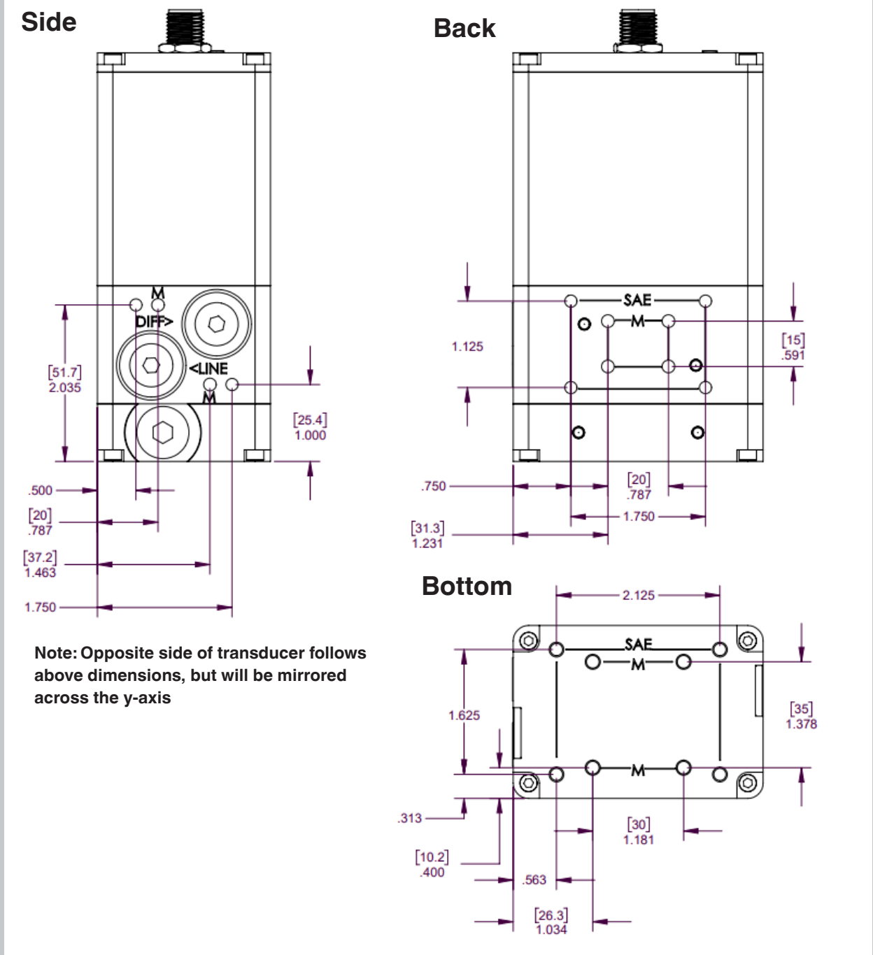
Figure 5.5B Mounting diagram with relief valve
